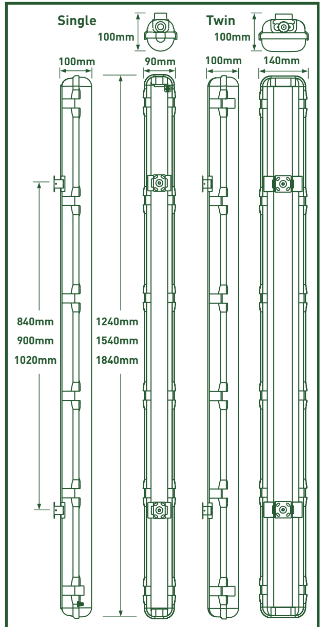
LEDs (Twin)
