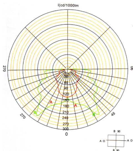
Fig 1: CIB 125 MV
